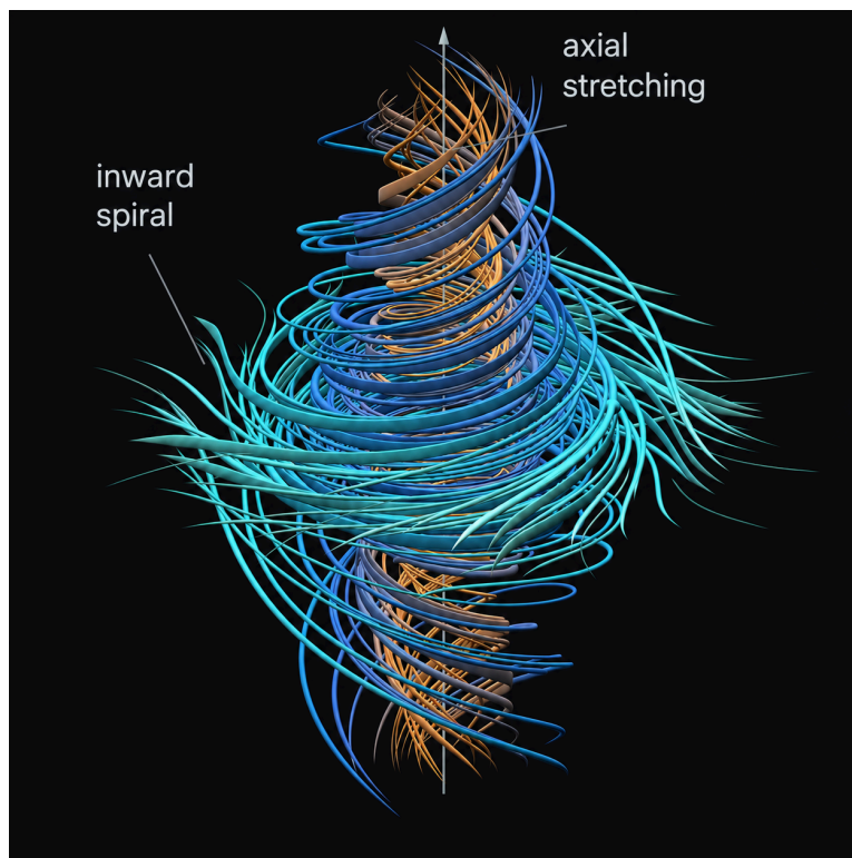
Figure 1: A collapsing vortex: trajectories spiral inward and stretch along the axis. Image: OpenAI.
